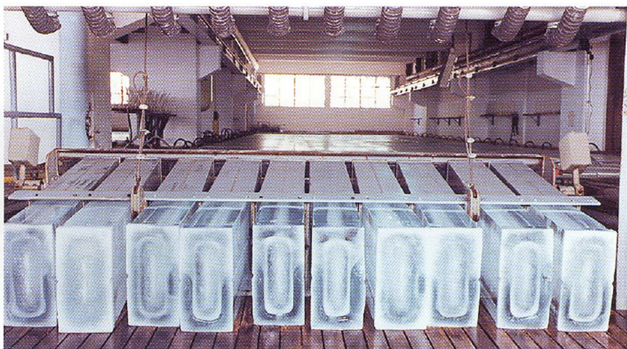
倒冰Ice tipping
