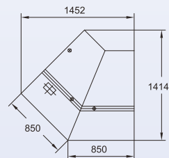
135°Outer corner
