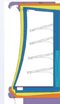
Sonyo double air curtain
