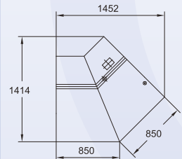
135°Inner corner
